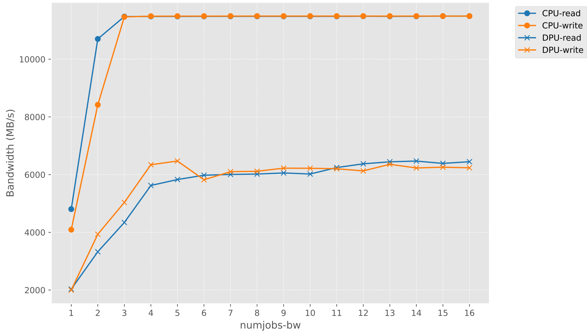
Bandwidth vs numjobs-bw
